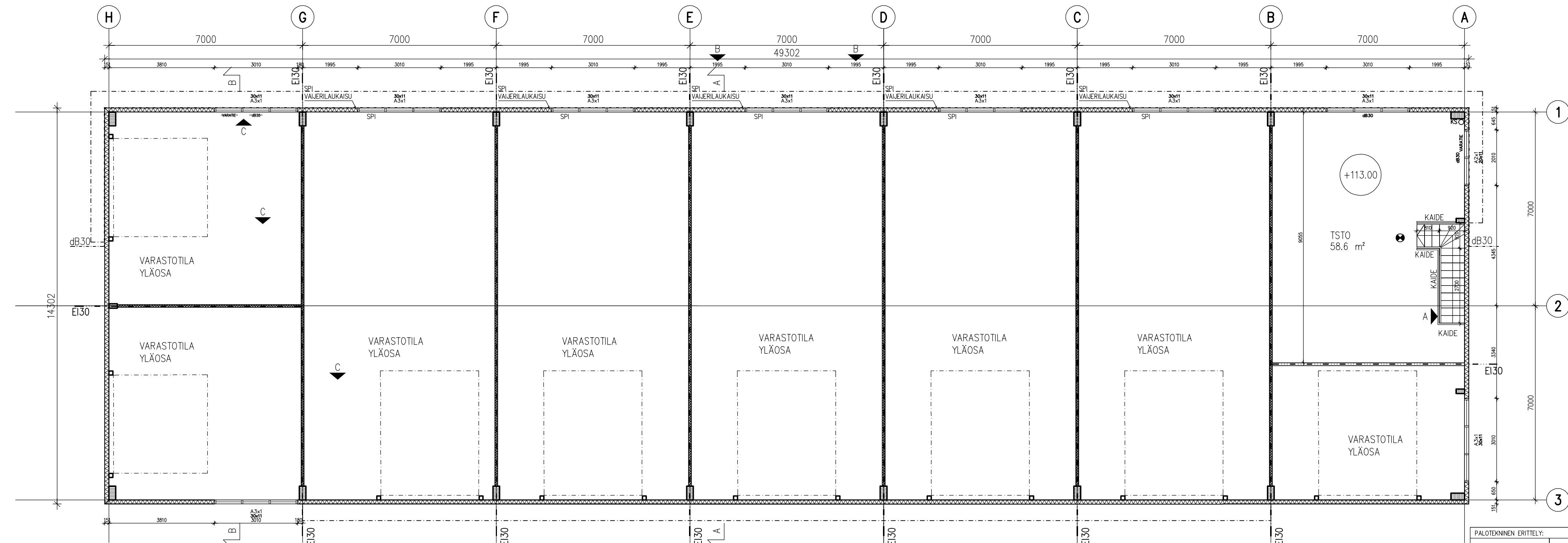
HALLI B/ 2.krs.
